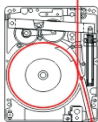
'O' Cable Guidance
